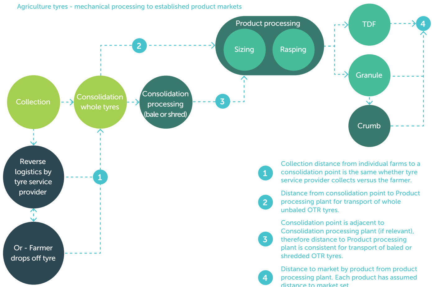
Figure 5: A recovery pathway for end-of-life OTR tyres from the Australian agriculture sector, for illustrative purposes only. Potential viability of one configuration of services and operations over others will depend on features that are individual to the catchment of OTR tyres. OTR tyre recovery in other countries
