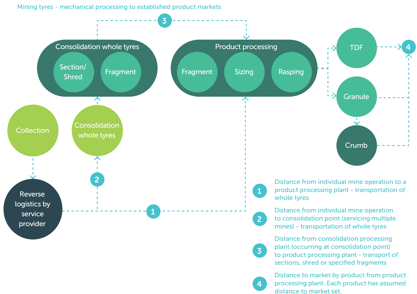
Figure 4: A recovery pathway for end-of-life OTR tyres from the Australian mining sector, for illustrative purposes only. Potential viability of one configuration of services and operations over others will depend on features that are individual to the catchment of OTR tyres.
