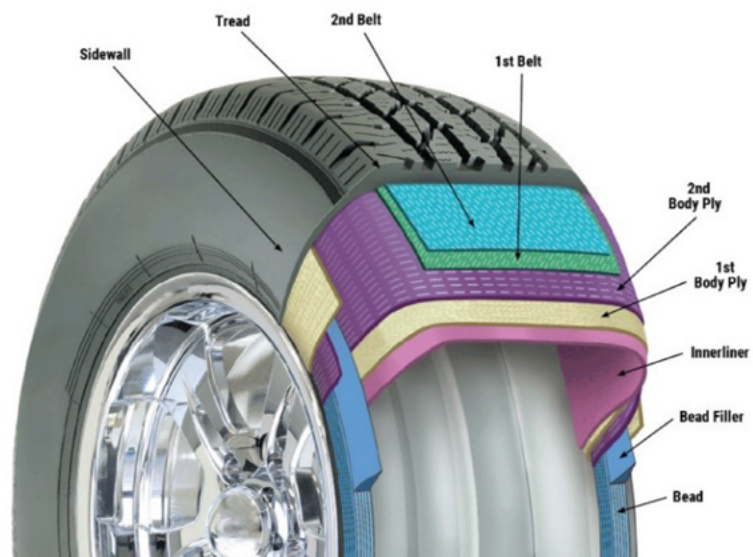
Figure 1: An example of the construction and typical components of a pneumatic tyre. 1
