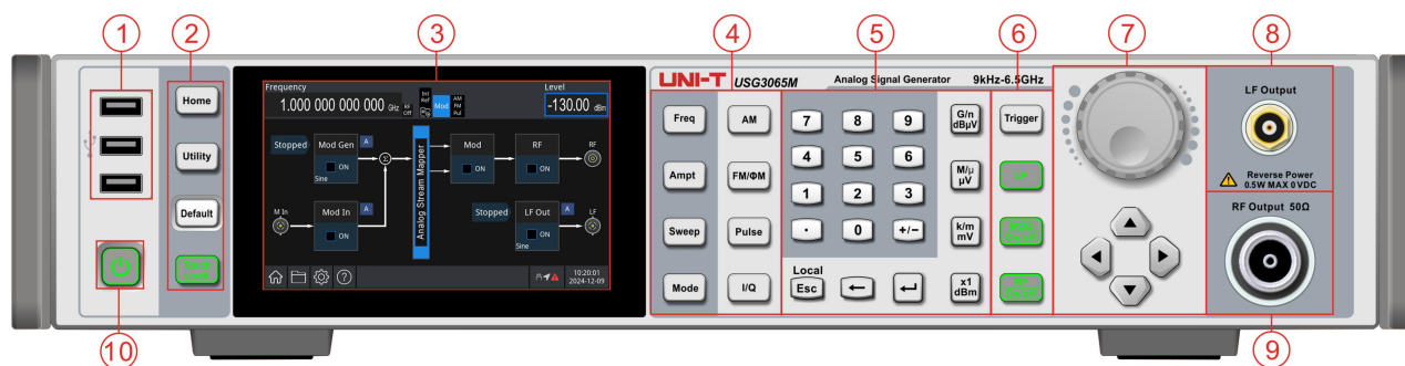
Front Panel
