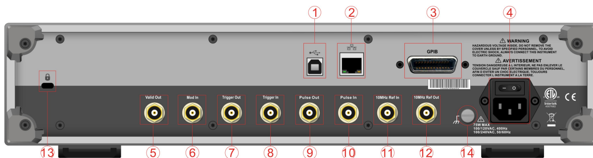
Rear Panel
