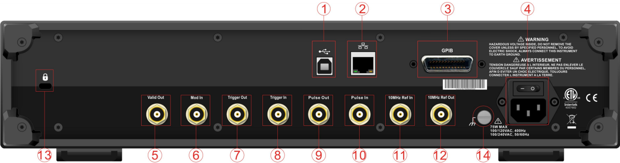
Rear Panel
