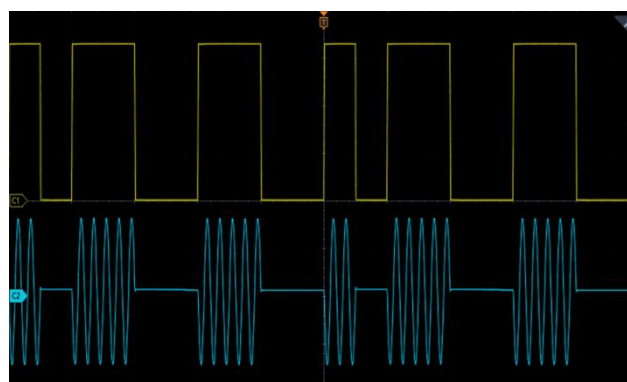
Measured Pulse Modulation Output
