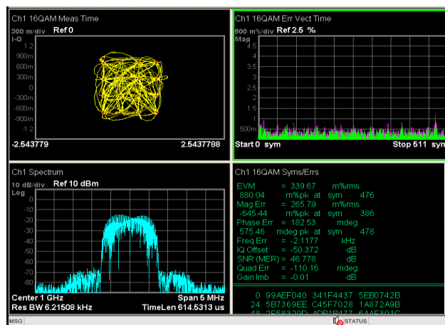
QAM16 Demodulated Signal Measurement
