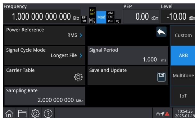
Multi-Carrier Modulation Settings Interface
