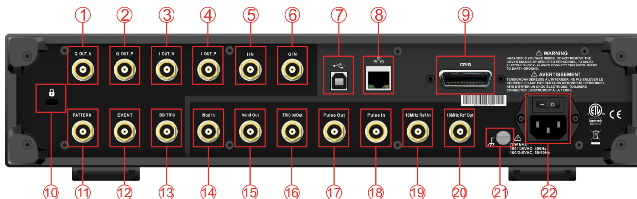
Rear Panel
