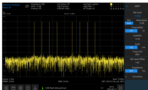
Multi-Tone Modulation Spectrum Display
