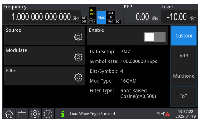
Digital Modulation Settings Interface
