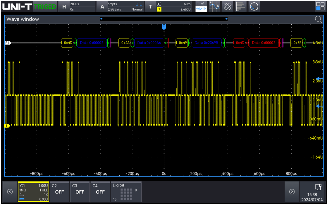
ARINC429 trigger and decoding
