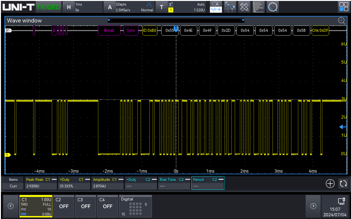
LIN trigger and decoding
