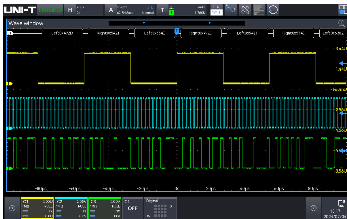
I2S trigger and decoding
