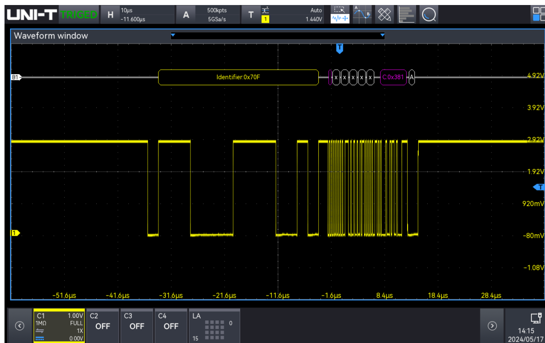
CAN-FD trigger and decoding
