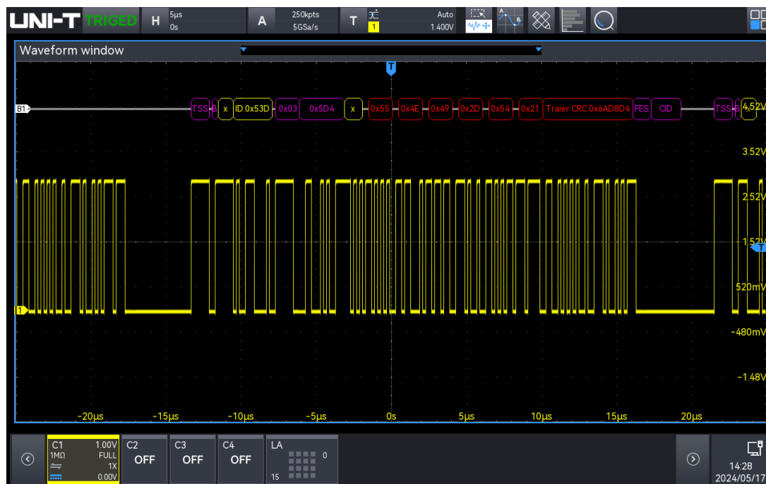
FlexRay trigger and decoding
