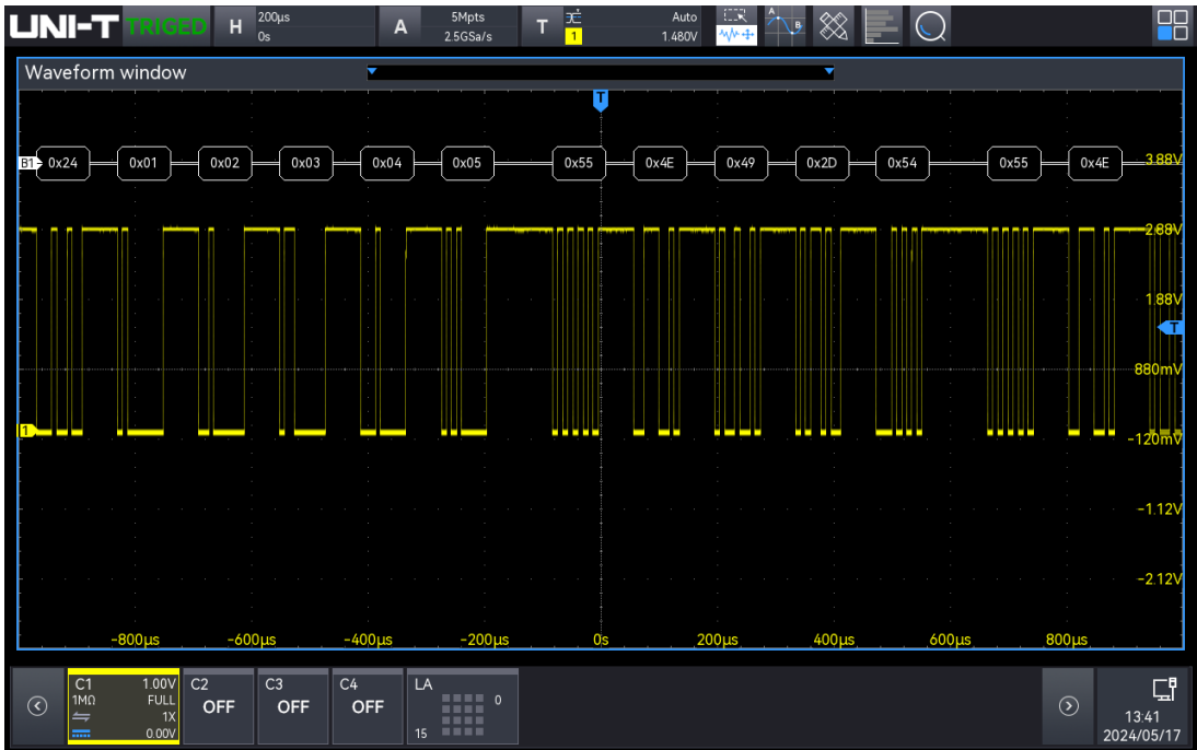
UART trigger and decoding
