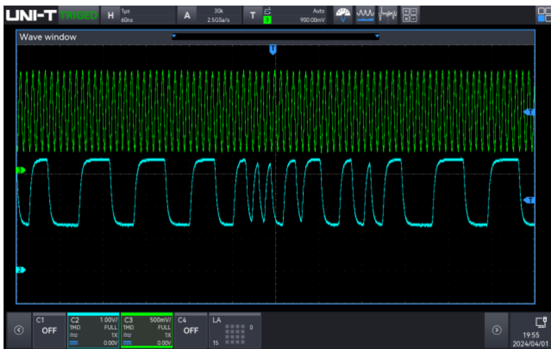
Setup & Hold signal
