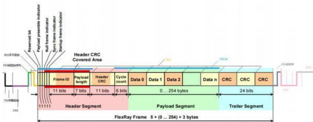
Figure 4-1: FlexRay frame format.
