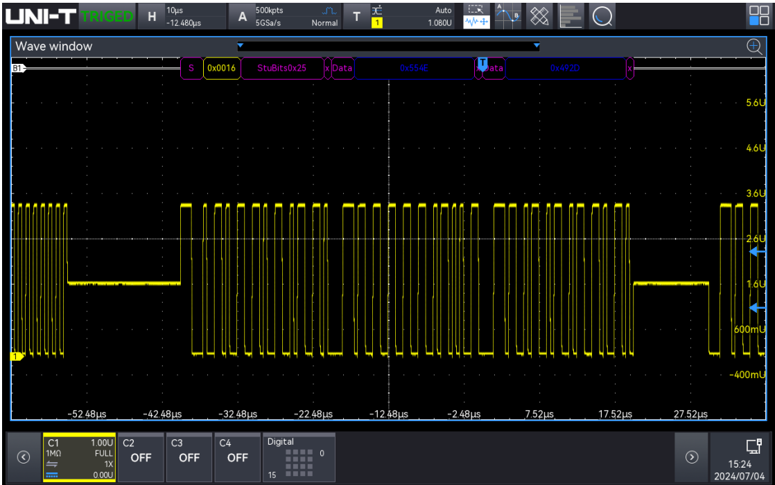
1553B data trigger and decoding
