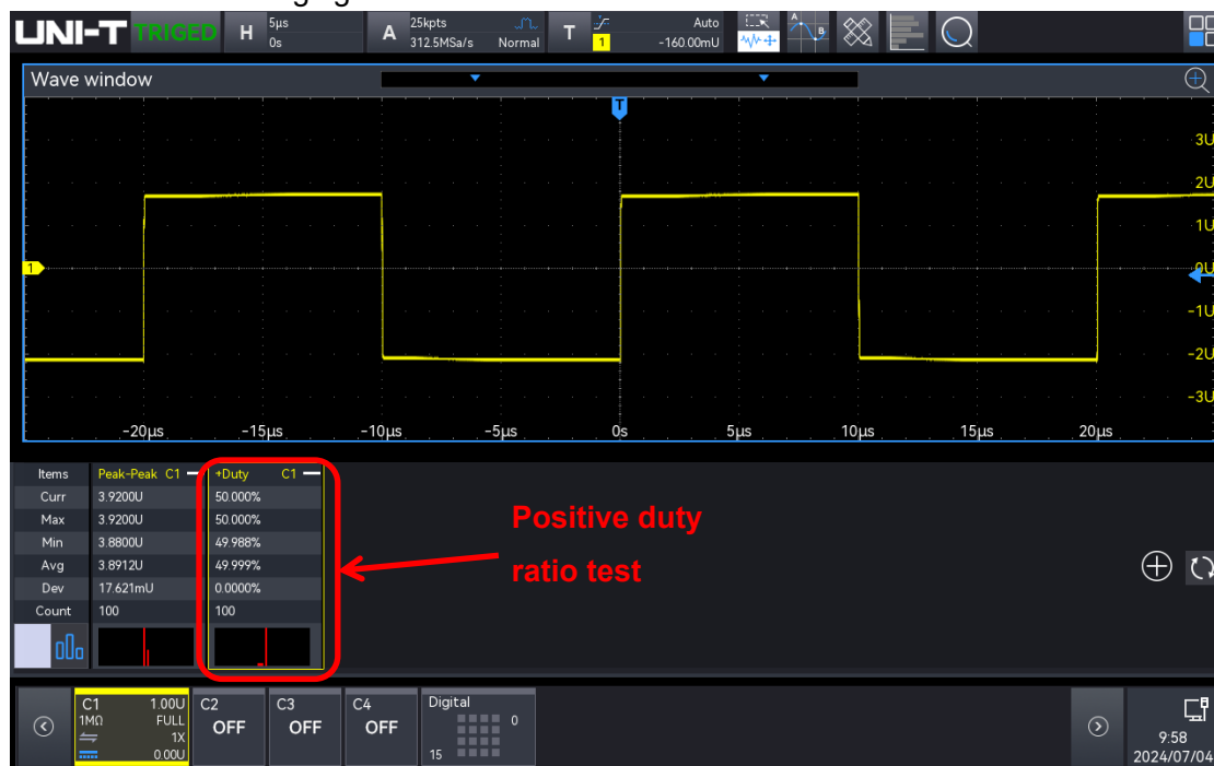
Demo result of square wave
