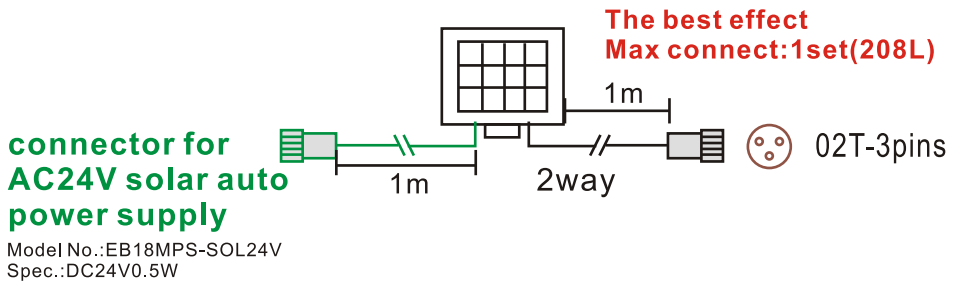
DC24V 0.5W solar panel
