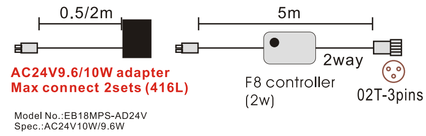
AC24V adapter
