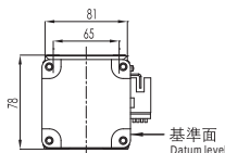
局部視圖B Local view
