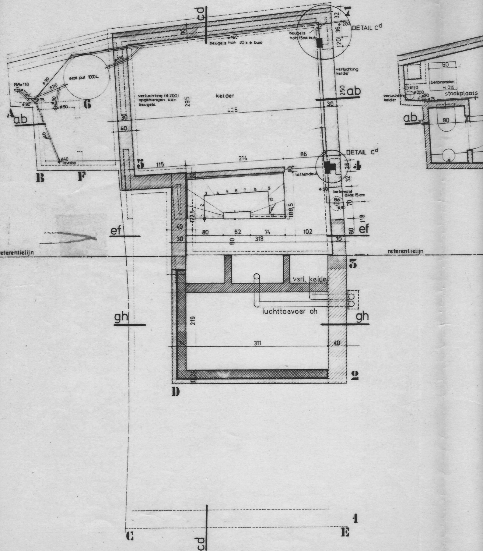
kelder-riolering-fund.
