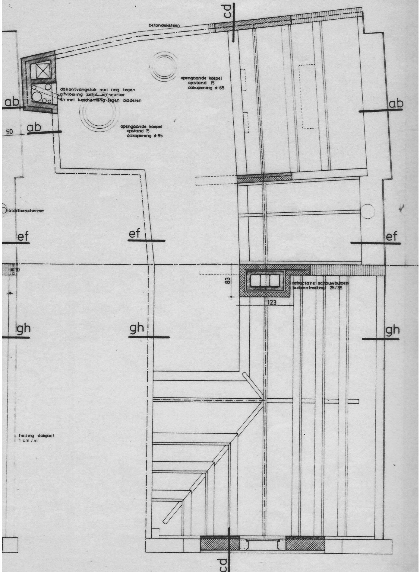
dakenplan
