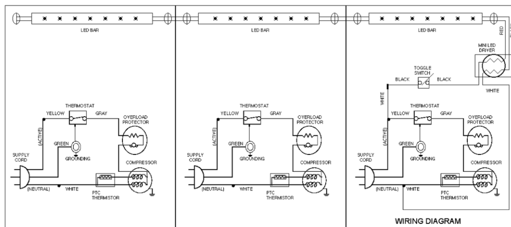
Electrical Wiring Diagram
