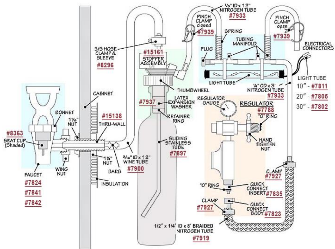
WineKeeper System Diagram
