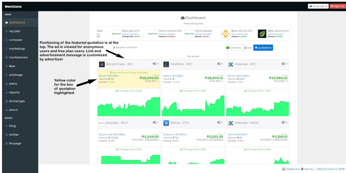
Screen: Dashboard
