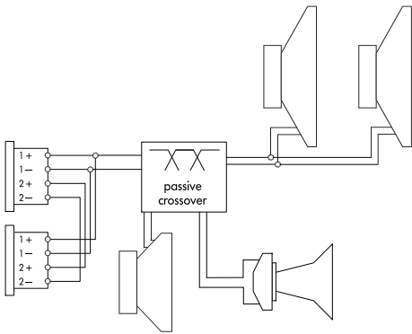
Connector wiring
