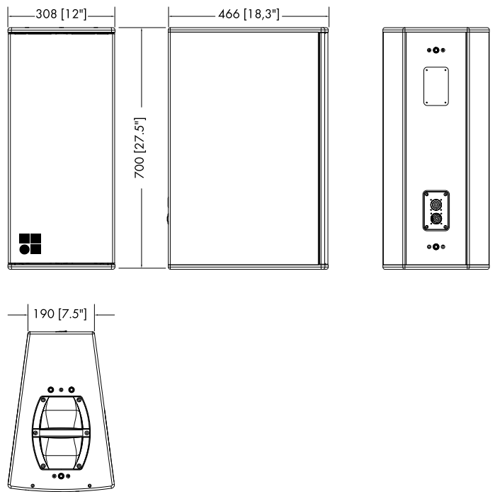
V7P/V10P cabinet dimensions in mm [inch]
