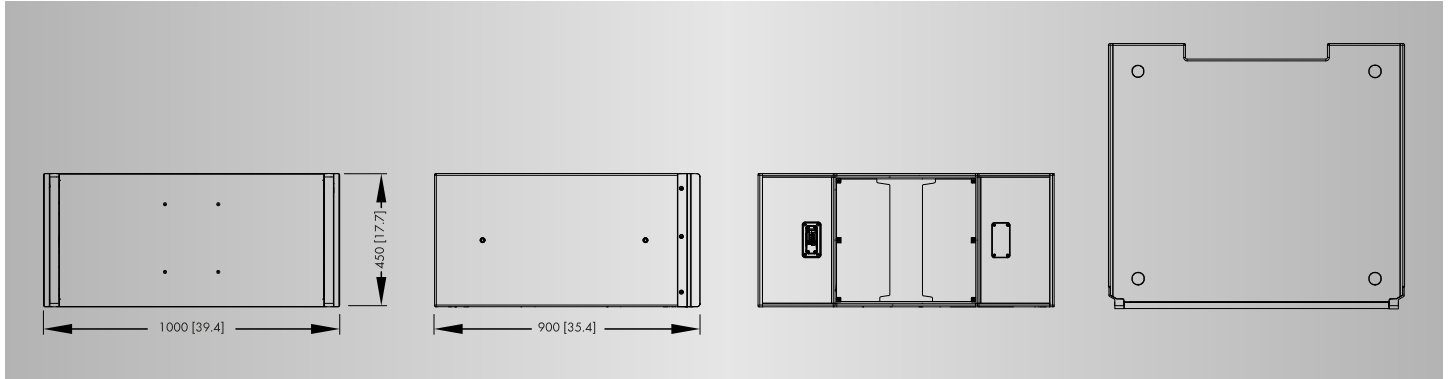
KSLi-GSUB cabinet dimensions in mm [inch]
