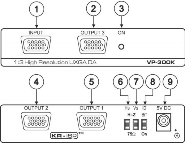
Figure 2: VP-300K 1:3 High Resolution UXGA DA
