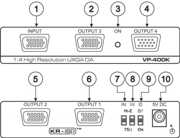
Figure 3: VP-400K 1:4 High Resolution UXGA DA
