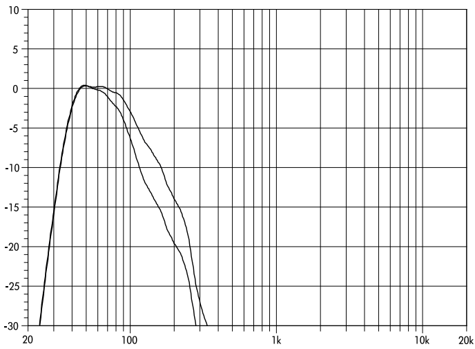
Fig. 2: V-SUB frequency response, standard and 100 Hz mode
