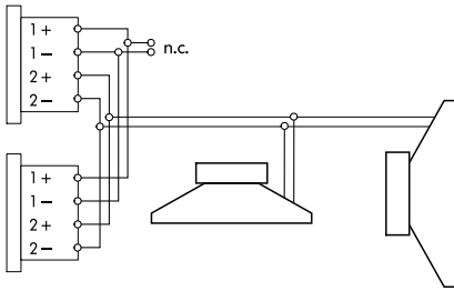
Fig. 1: Connector wiring
