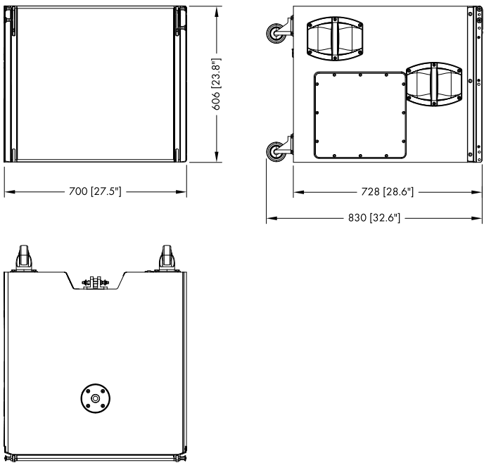
Fig. 3: V-SUB cabinet dimensions in mm [inch]
