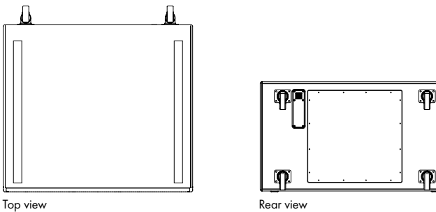
J-INFRA cabinet dimensions in mm (inch)
