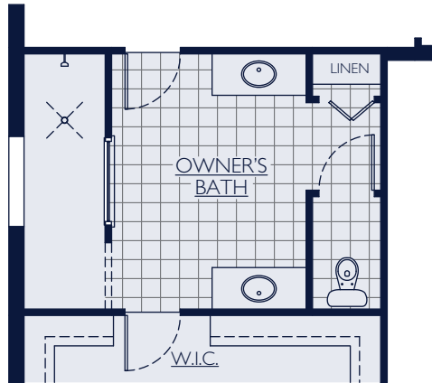
OPT. OWNER'S BATH ROMAN SHOWER
