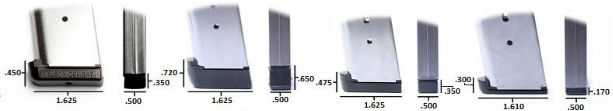
47BN Standard Base Pad Polymer
