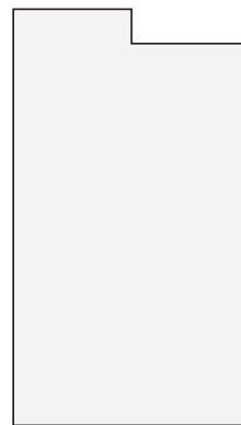
Notches minimum 3/8" inside radius for satin finish minimum 2-1/2" inside radius for polished finish
