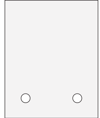
Round Holes Holes must be located at least 2.5 x hole diameter from the edge. For example, a 2" hole must at least be located 5" away from the glass edge.
