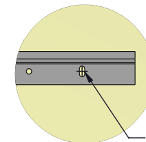
DETAIL A SCALE 1 : 5 VERTICAL DIMENSIONS ARE TO CENTER OF MOUNTING SLOTS
