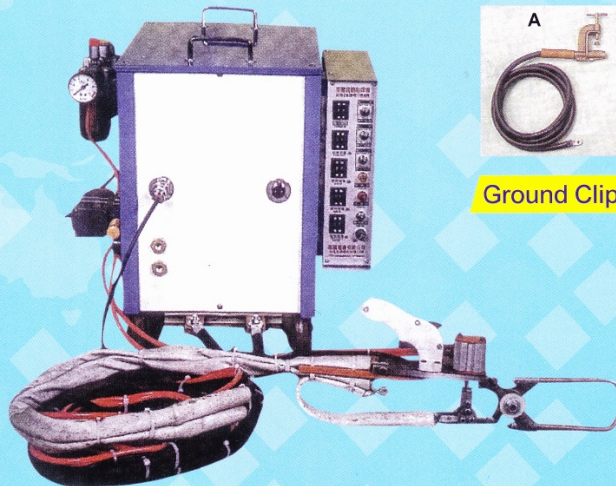
Pneumatic Clipper Type Spot Welder 氣動夾式點焊機
