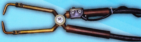
Manual Clipper Welder Head 手動夾式點焊頭
