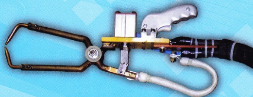
Pneumatic Clipper Welder Head 氣動夾式點焊頭
