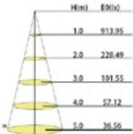
Illuminance at a Distance
