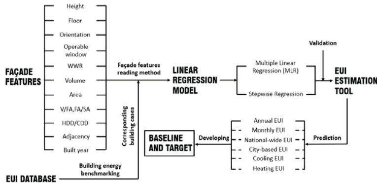
Figure 2: Methodology.
