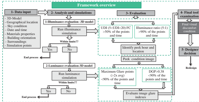
Figure 2: Framework overview
