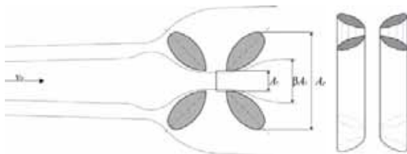
Figure 6: Combined Plate Concentrator at \varphi = 45^\circ . Adopted from (Mertens, 2006)
