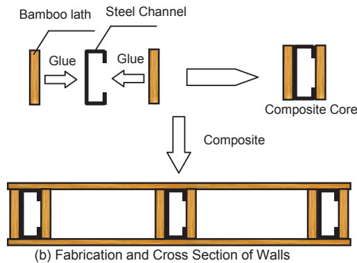
(b) Fabrication and Cross Section of Walls
