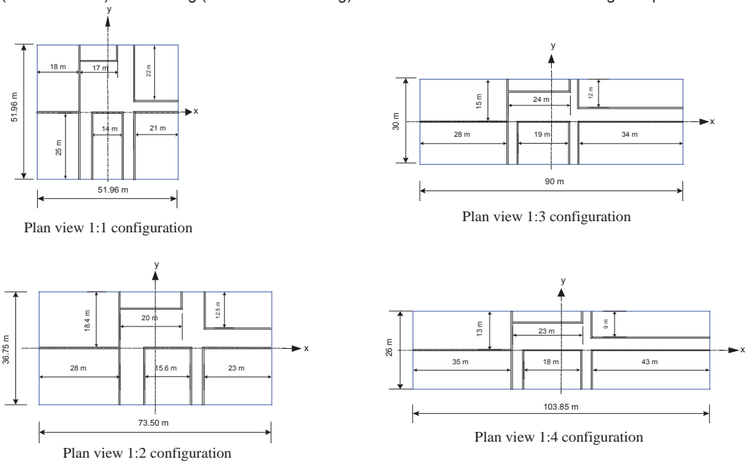
Figure 2: Footprint aspect ratios for modeled buildings in plan view.
