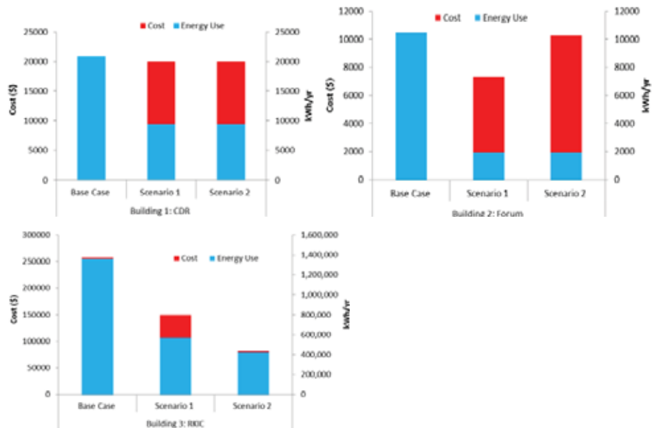
Figure 3: Energy use versus cost in each case.
