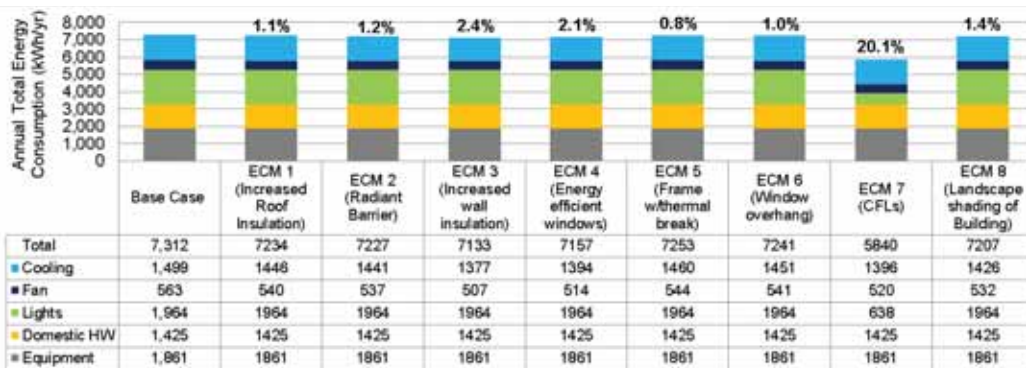
Figure 5: Annual total site energy consumption of individual ECMs: on-grade construction (Upper) and elevated slab construction (Below).
