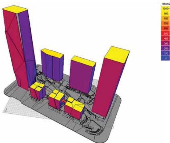
Figure 11: Envelope Insolation, Guangzhou poly mixed use project
