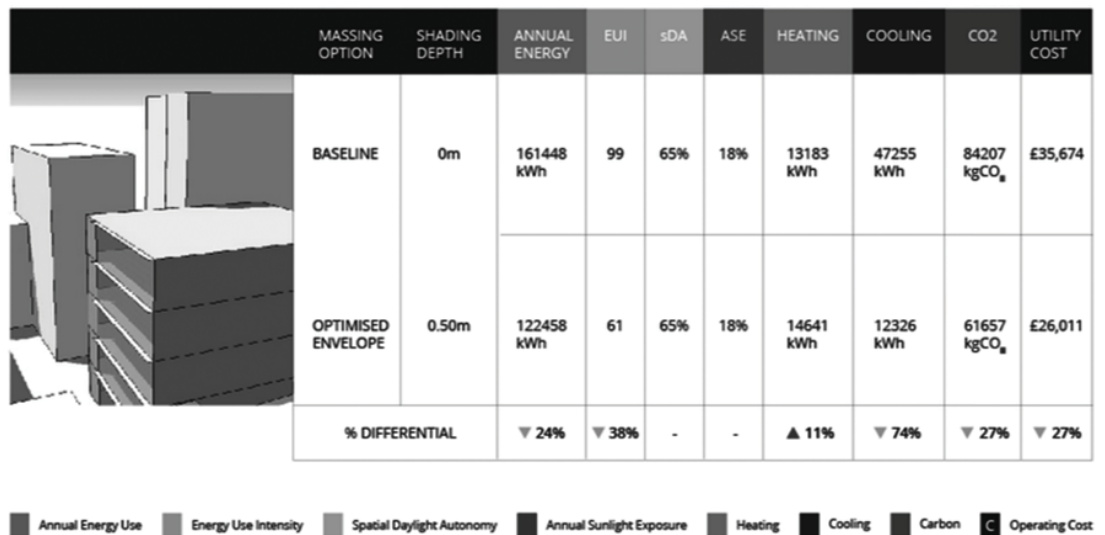
Figure 1: Baseline vs. Optimized Building Comparison: A representation of analysis results from Sefaira, showing the savings offered by an optimized envelope. (Sefaira Inc., 2014)
