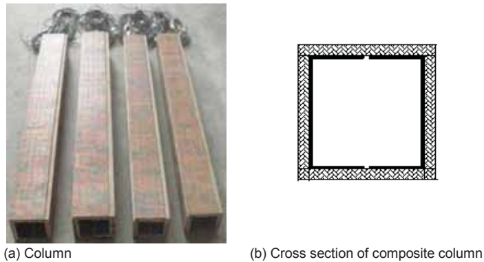
Figure 4: Bamboo-steel composite column.
