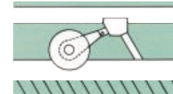
Carman's positive arm drive compensates for load surges and other out-of-phase forces.
