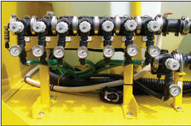
Pressure Regulator For Spray Head
