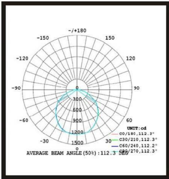
Light Distribution Graph:
