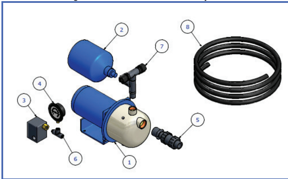
Figure EEEE: Pressure Modification System
