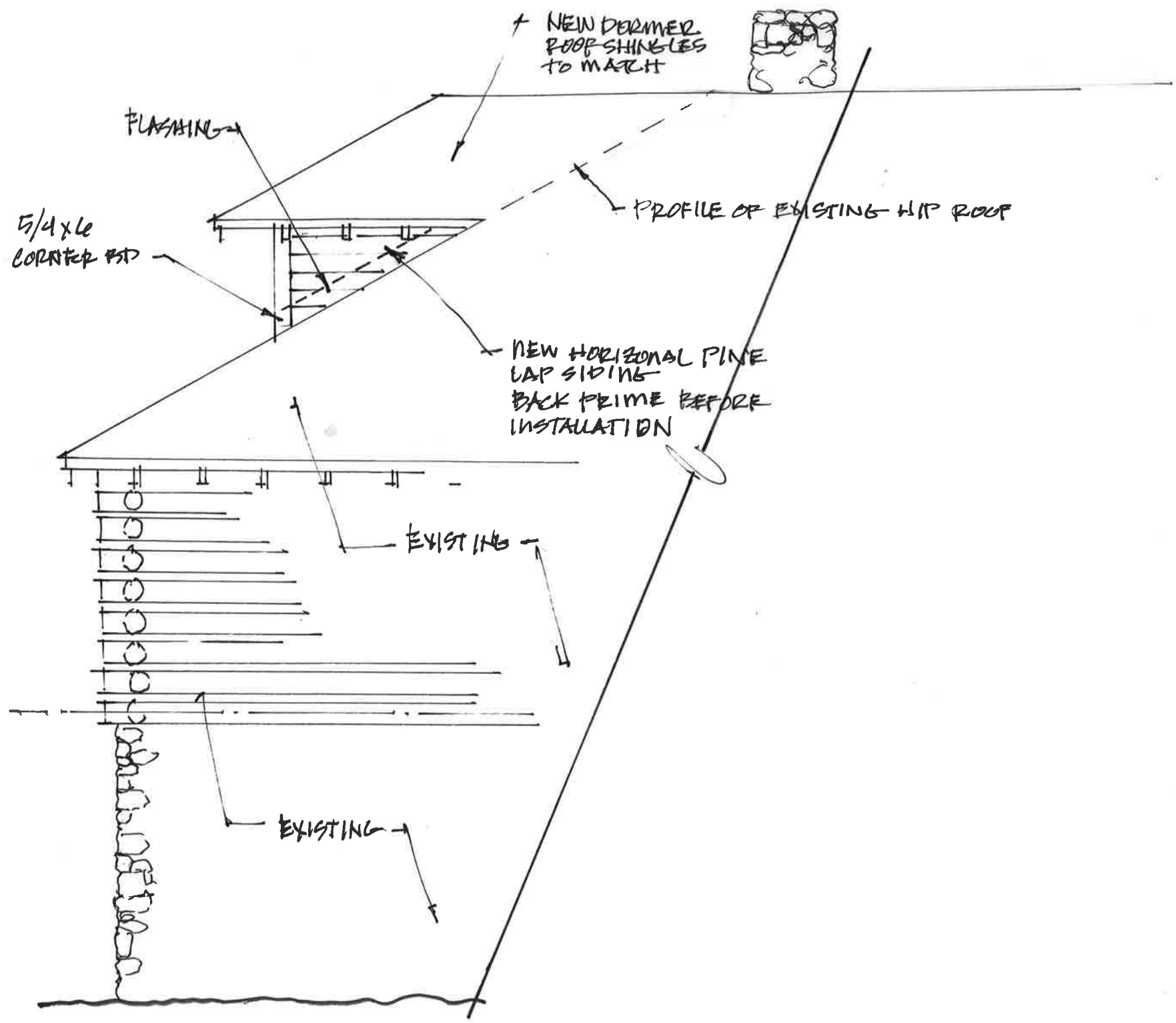
PARTIAL SIDE ELEVATION 1/4" = 1'-0"
