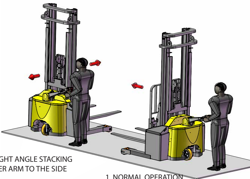
1. NORMAL OPERATION REAR WHEEL PARALLEL WITH TILLER ARM
