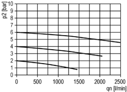
flow characteristic
