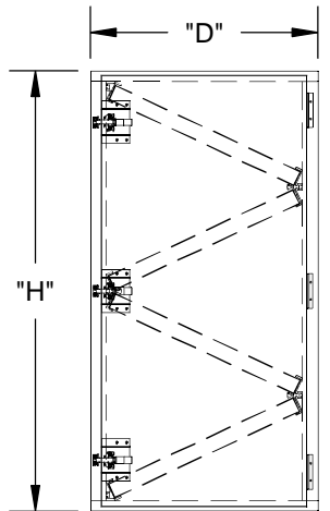
ACCESS VIEW
