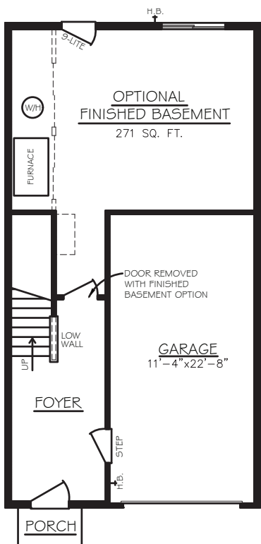
LOWER LEVEL
