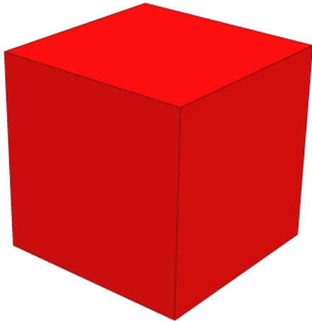
cuubo
