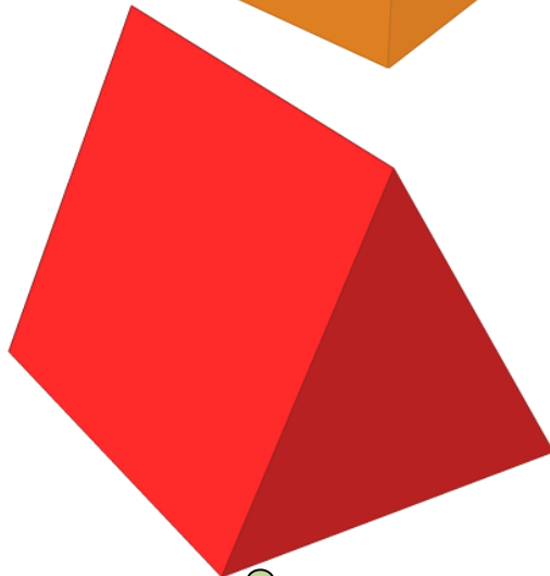
prisma triangular
