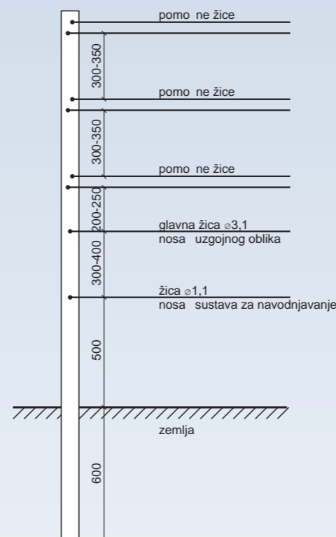
detalj armature
