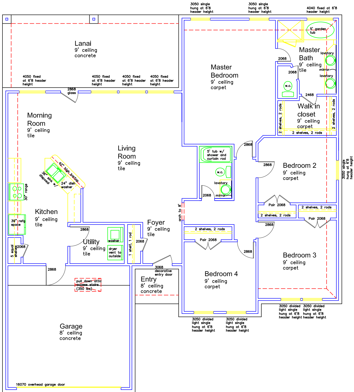
Floor Plan # 2500 GABLE
