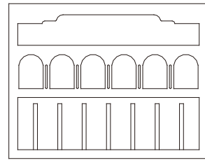
80/90 Wine Rack (Elevation) D32 × W80 × H70
