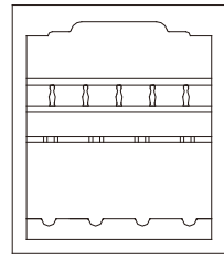
60/80 Wine Rack (Elevation) D32 × W60 × H70
