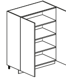
2 doors, shelves w 35 7/16", 47 1/4"
