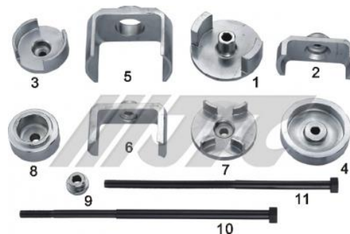
JTC-4101 BENZ SUB-FRAME BUSH INSTALLER / REMOVER (WW221)
