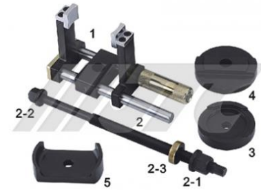
JTC-4096 BMW SUSPENSION BUSH EXTRACTOR / INSTALLER (E39)
