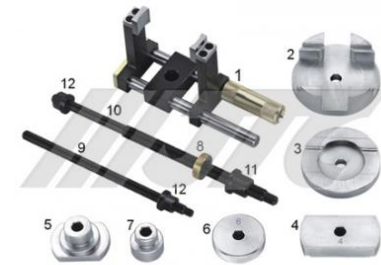
JTC-4161 BENZ SUB-FRAME BUSH INSTALLER / REMOVER (W210)
