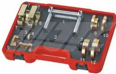
JTC-4242 BMW REAR SUSPENSION BUSH REMOVER / INSTALLER KIT (E87, E90)
