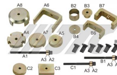
JTC-4203 BENZ SUB-FRAME BUSH INSTALLER / REMOVER (W211)
