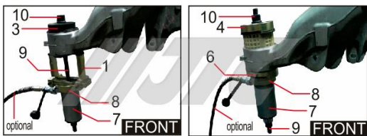
removal: 1, 3, 7, 8, 9, 10 installation: 4, 6, 7, 8, 9, 10
