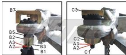
INSTALL FRONT BUSH
