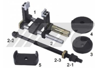
JTC-4096 BMW SUSPENSION BUSH EXTRACTOR / INSTALLER (E39)
