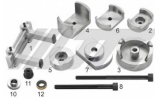
JTC-4334 BENZ SUB-FRAME BUSH INSTALLER / REMOVER (W204)
