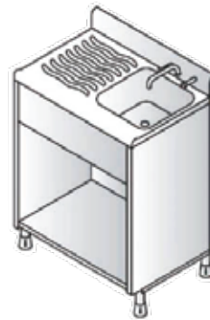
Stainless Steel Single Sink With Beer Station AMP400-1 Dimension: 800 X 500 x 850 +100mm AMP400-2 Dimension: 1000 X 500 x 850 +100mm
