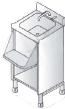
Stainless Steel Single Sink Workstation AMP399-1 Dimension: 600 X 500 x 850 +100mm AMP399-2 Dimension: 800 X 500 x 850 +100mm AMP399-3 Dimension: 1000 X 500 x 850 +100mm
