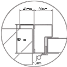
Frame dimensions
