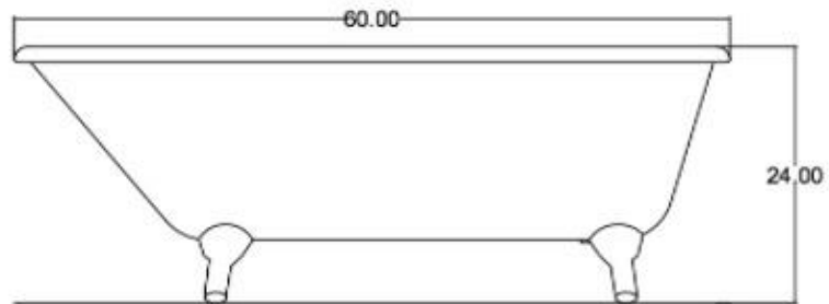
Side View
