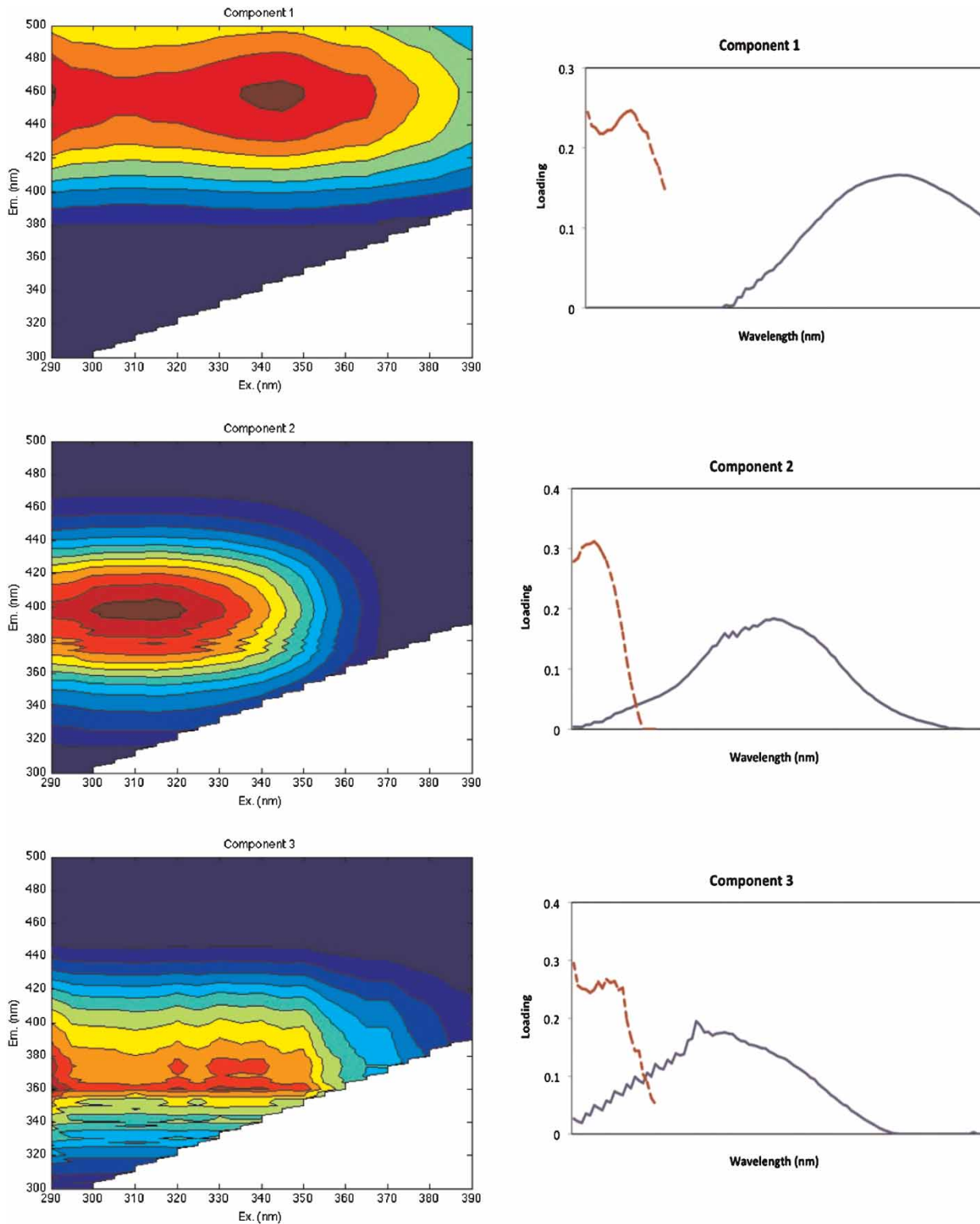
Figure 5 | Fluorescence signatures of three identified PARAFAC model components. Contour plots present spectral shapes of excitation and emission of derived components. Line plots adjacent to each contour plot present split-half validation results for each identified component. Excitation (dotted line) and emission (solid line) loadings for each component, obtained from two independent PARAFAC models on random halves of the data array.
