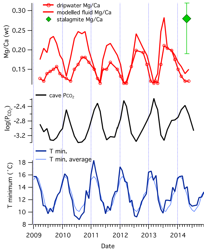
Fig. 7. Forward modelled fluid Mg/Ca compared with dripwater Mg/Ca, cave air \text{PCO}_2 and minimum temperature (expressed as monthly mean of daily minimums) for our low-flow site (site 1A). The Mg/Ca ratio measured on the top of the stalagmite collected underneath this drip site is also shown. This value is converted to the equivalent in fluid Mg/Ca for comparison and is bracketed by the range of values measured within the upper 1.5 mm of calcite, estimated to have precipitated within the last two decades, although our age model for this stalagmite is incomplete. Our forward-modelled fluid Mg/Ca represent maximum values when equilibrium is fully attained. Thus similar values would arise if we forward-modelled our high-flow data since our reverse-modelling showed that both solutions initially equilibrated with similar \text{PCO}_2 values. In practice, for our high-flow site, this end-member may represent cave pools at the end of the flowline. Comparison of stalagmite crest and flanks can indicate how close to the end-member a particular stalagmite has reached.
