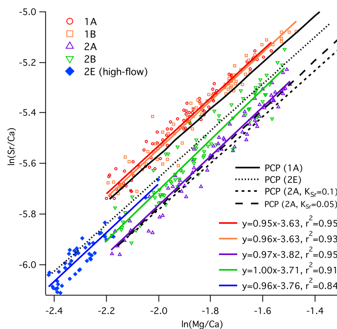
Fig. 4. Dripwater \ln(\text{Sr}/\text{Ca}) versus \ln(\text{Mg}/\text{Ca}) (weight ratio) data, with linear fits for each site, plus calculated PCP trendlines for sites 1A, 2E and 2A. PCP trendline for site 2A is shown twice, using K_{\text{Sr}} = 0.1 and K_{\text{Sr}} = 0.05 , see text in section 4.3. See Methods for PCP trendline calculation.
