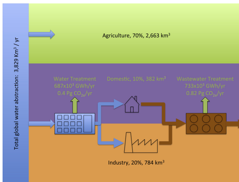
Fig. 1 – Energy consumption and \text{CO}_2\text{e} emissions associated with global water and wastewater treatment. (Abstraction figures from UNESCO (2009). Energy calculations based on 48.22% surface water at 0.371 \text{ kWh/m}^3 , 48.23% groundwater at 5 \text{ kWh/m}^3 and 3.55% desalination at 5 \text{ kWh/m}^3 (EPRI, 2002; WaterUK, 2010). \text{CO}_2\text{e} emissions based on 0.34 and 0.7 tonnes/Ml for water and wastewater treatment respectively (WaterUK, 2010).
