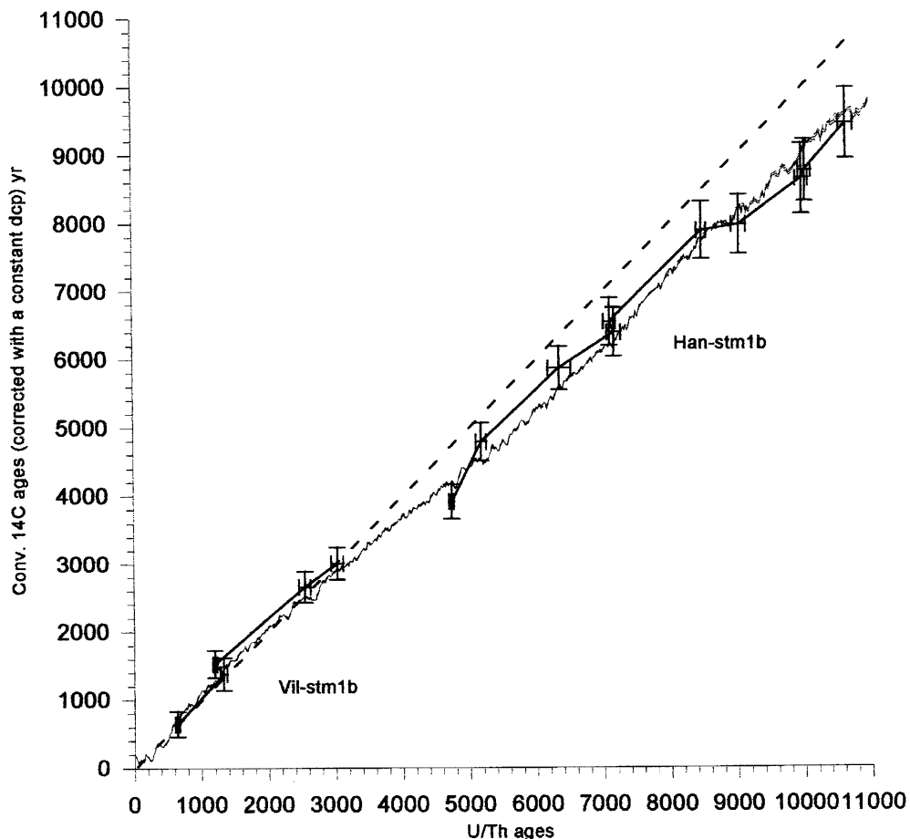
Figure 5 Comparison of conventional 14 C ages (dcp corrected), U/Th ages (of Han-stm1b and Vil-stm1b stalagmites), and calibration curve from dendrochronology (Stuiver and Kra 1986). Note the good fit between our measurements and the calibration curve.
