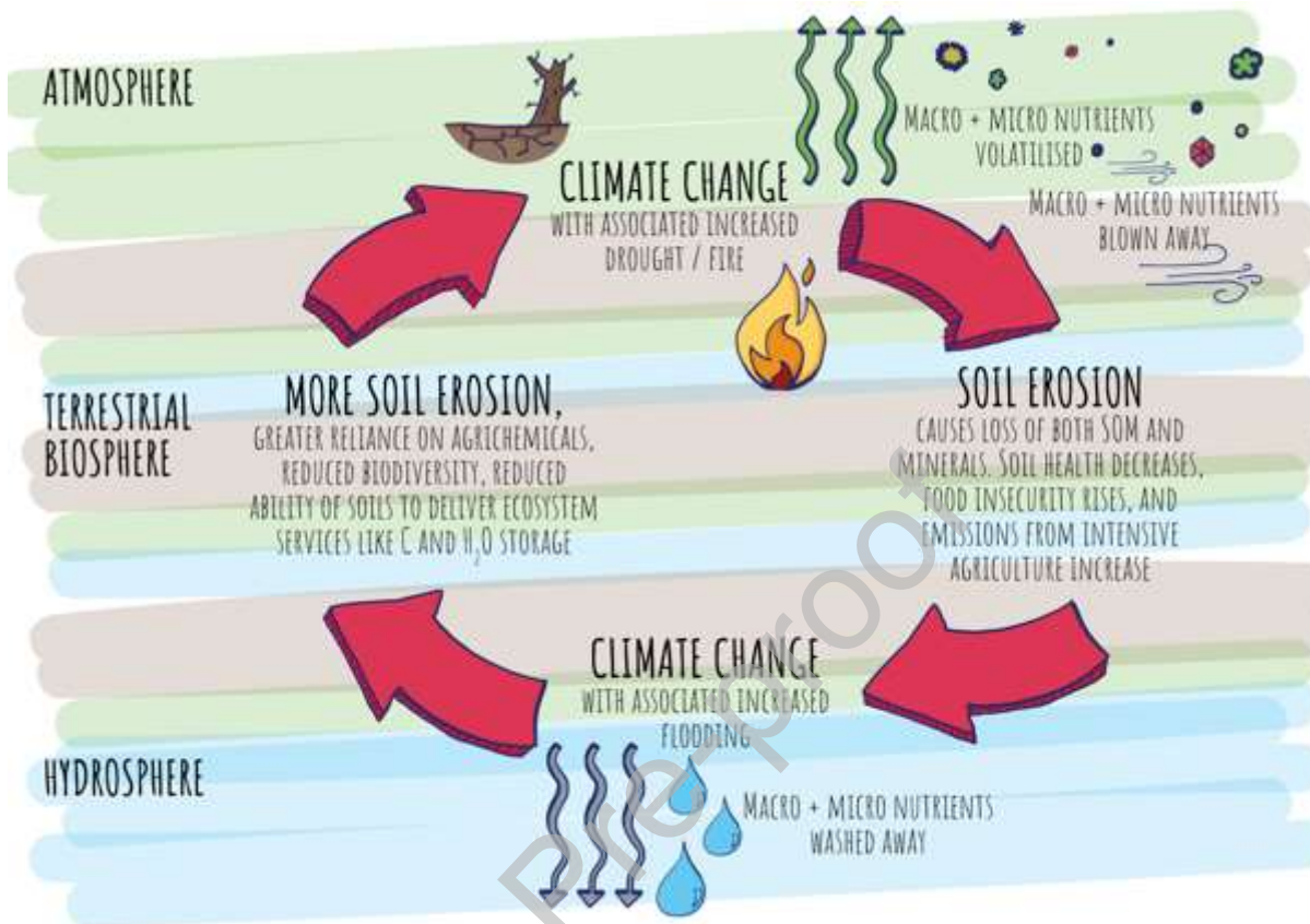
Figure 2 - Vicious cycle of soil degradation and climate change - where the already degraded soil (due to land mismanagement by communities and intensive agricultural practices) is in a negative feedback loop with the extreme flooding and drought/fires caused by climate change. Both organic and inorganic components of soil are literally washed away under flooding, blown away under drought and damaged under severe wildfires which can contribute to greenhouse gas emissions. However, the biggest link between soil degradation and climate change is that soil degradation leads to overuse of agrochemicals in conventional intensive agriculture which not only directly feeds global greenhouse gas emission but further decreases soil biodiversity, exacerbating soil degradation and increasing soil's vulnerability to the extremes of flooding and drought/fire.
