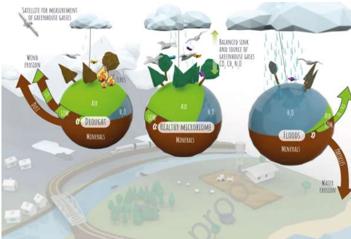
Figure 3. Healthy soil has a circular economy where inputs and outputs of C and N and other macro and micro nutrients are balanced. SOM is central to the living soil. Many soil functions and SOM turnover and production of the GGH \text{CO}_2 , \text{CH}_4 and \text{N}_2\text{O} is/are related to both water content and redox, both of which are related to soil structure. We highlight here the role of minerals in SOC stabilisation (one of the key controls on SOC accessibility) and therefore soil structure, as well as the circle of SOC degradation and climate change represented by the Newton's cradle configuration representing the link between healthy soil (centre where soil has natural cycle of balanced inputs and outputs – see Figure 1) and degraded soils (as represented by more outputs than inputs of both solid particles and gases) under extreme drought (LHS) and flood conditions (RHS) caused by climate change. The satellite represents future soil health data collection via satellite technology.
