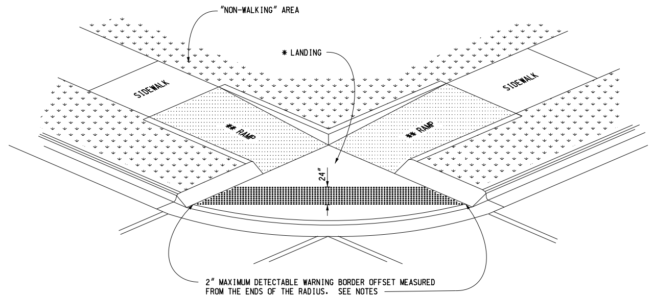
(TANGENT DETECTABLE WARNING SHOWN)
