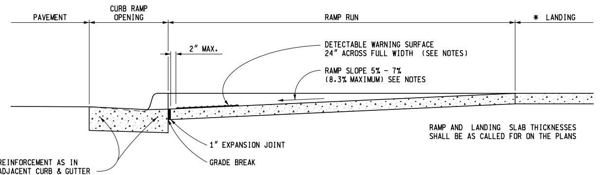
SIDEWALK RAMP TYPE RF (ROLLED / FLARED SIDES)
