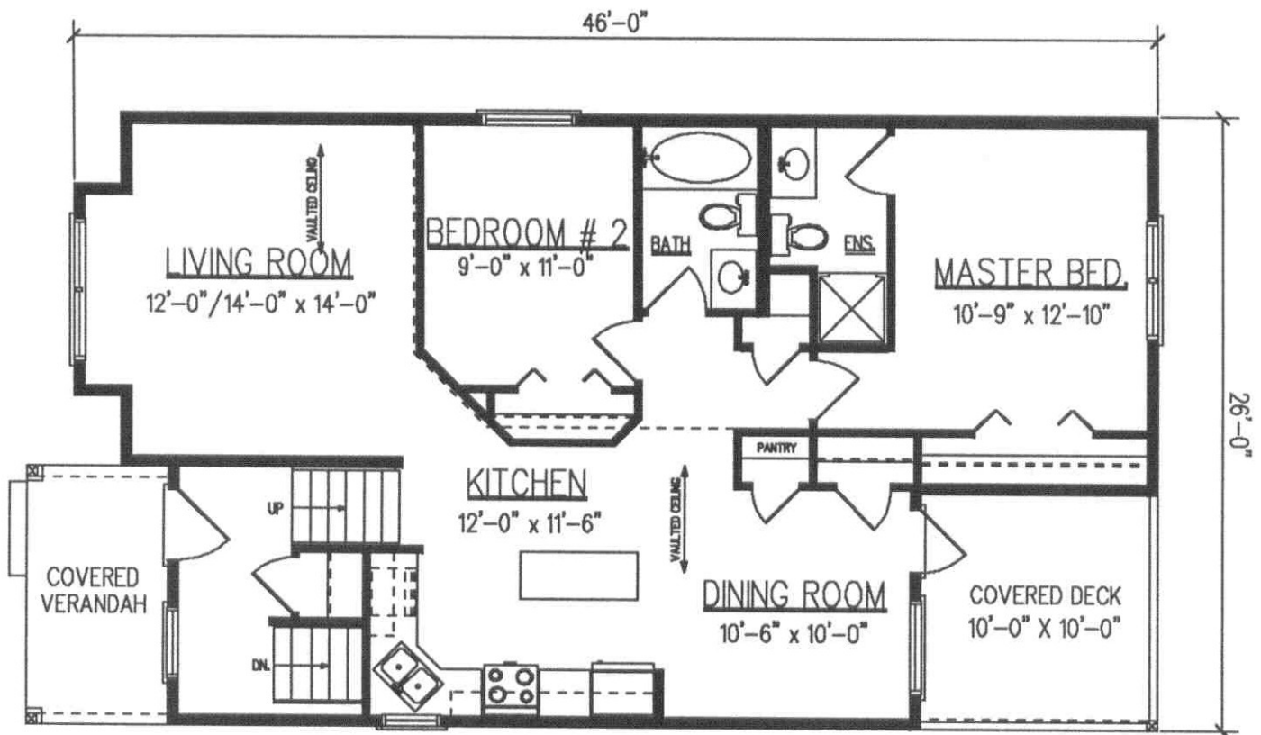
FLOOR PLAN 1040 SQ. FT.
