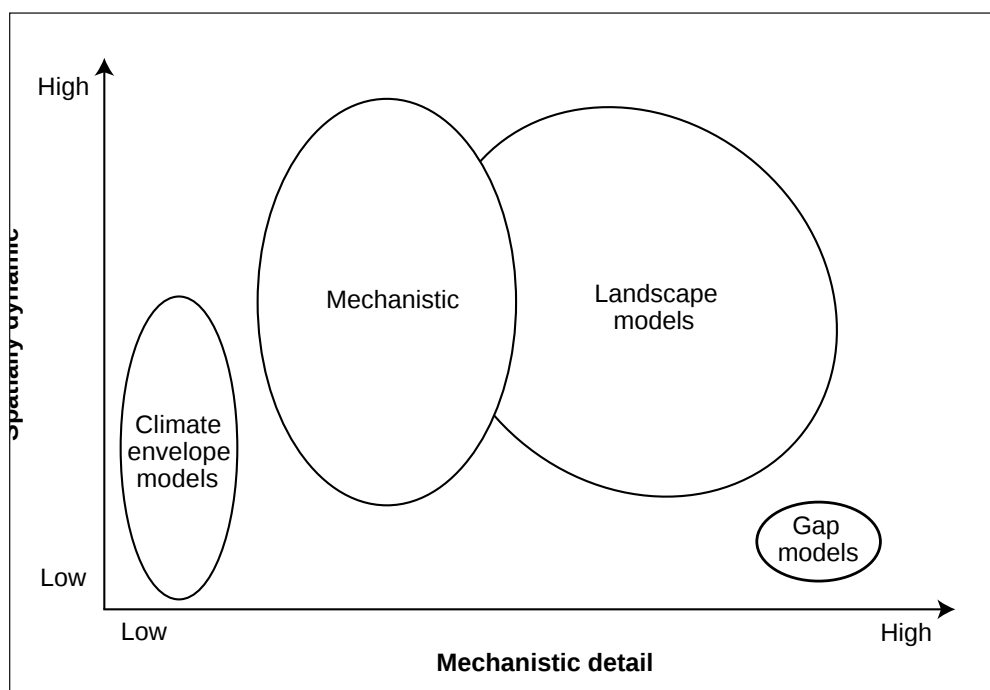
Figure 2—Conceptual diagram of the relative emphasis on spatial dynamics and mechanistic (process-based) detail in different types of models used to understand the effects of climate change. After Mladenoff (2004).
